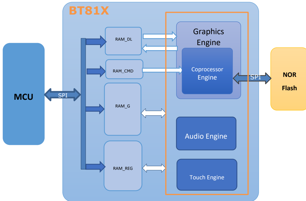
Figure 1 – BT81X data flow
